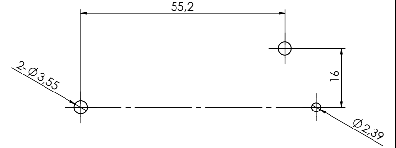
PCB LAYOUT
